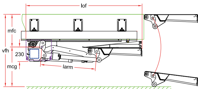
Truck / DH-SM.20
